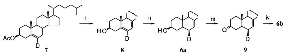
Scheme 2. Synthesis of [3\alpha,6\beta\text{-}^2\text{H}_2] lathosterol. Reagents and conditions: (i) NBS; \text{Bu}_4\text{NBr} , \text{Bu}_4\text{NF} ; \text{KOH-MeOH} (32%), (ii) Raney Ni (91%), (iii) PCC (91%), (iv) \text{LiAlD}_4 (71%).
