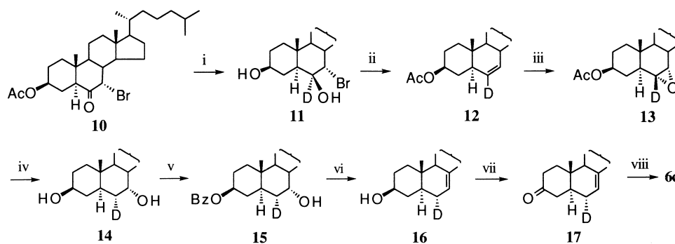
Scheme 3. Synthesis of [3\alpha,6\alpha-^2\text{H}_2] lathosterol. Reagents and conditions: (i) \text{LiAlD}_4 (34%), (ii) \text{Zn} , \text{AcOH} ; \text{Ac}_2\text{O}/\text{Py} (81%), (iii) \text{mCPBA} (99%), (iv) \text{LiAlH}_4 (100%), (v) \text{BzCl}/\text{Py} (73%), (vi) \text{POCl}_3/\text{Py} ; \text{KOH} , \text{MeOH} (38%), (vii) \text{PCC} (71%), (viii) \text{LiAlD}_4 (86%).
