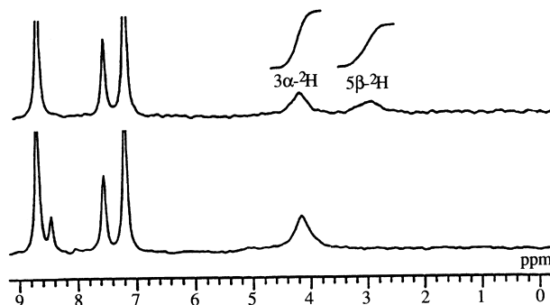
Figure 1. The ^2\text{H} -NMR spectra (77 MHz, pyridine) of 20-hydroxyecdysone ( 1 ). Top: derived from [3\alpha,6\beta-^2\text{H}_2] lathosterol ( 6b ); Bottom: derived from [3\alpha,6\alpha-^2\text{H}_2] lathosterol ( 6c ). The three intense signals at \delta 7.19, 7.56 and 8.69 are those of the solvent.
