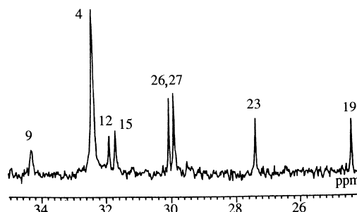
Figure 2. The ^{13}\text{C} -NMR spectrum (100 MHz, pyridine- d_5 ) of 20-hydroxyecdysone ( 1 ) derived from [4-^{13}\text{C}] -7-dehydrocholesterol.
