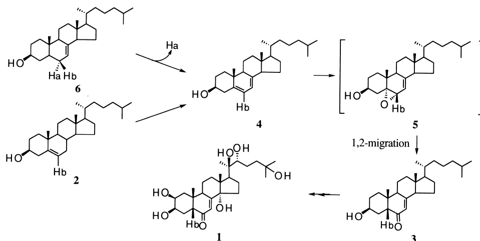
Scheme 1. Conversion of cholesterol ( 2 ) and lathosterol ( 3 ) into 20-hydroxyecdysone ( 1 ) via 7-dehydrocholesterol in Ajuga hairy roots with 1,2-shift of hydrogen (Hb) from C-6 to C-5.
