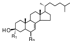
6a: \text{R}_1=\text{H} , \text{R}_2=\beta\text{-}^2\text{H} 6b: \text{R}_1=^2\text{H} , \text{R}_2=\beta\text{-}^2\text{H} 6c: \text{R}_1=^2\text{H} , \text{R}_2=\alpha\text{-}^2\text{H}
